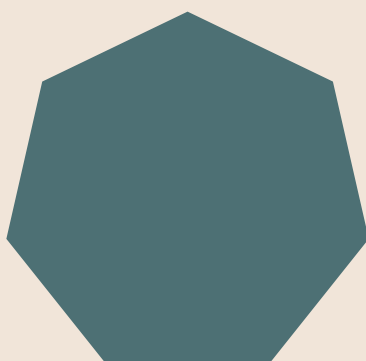
Heptagon
