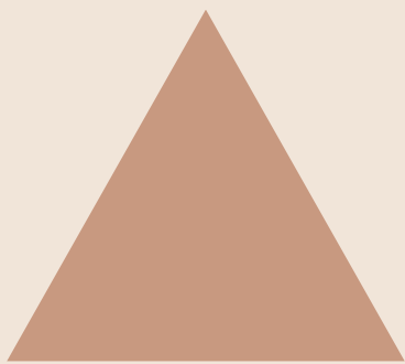
Triangle
