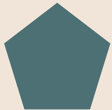
Pentagon
