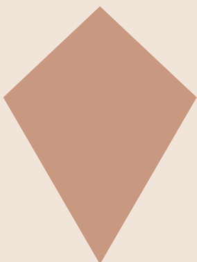
Kite
